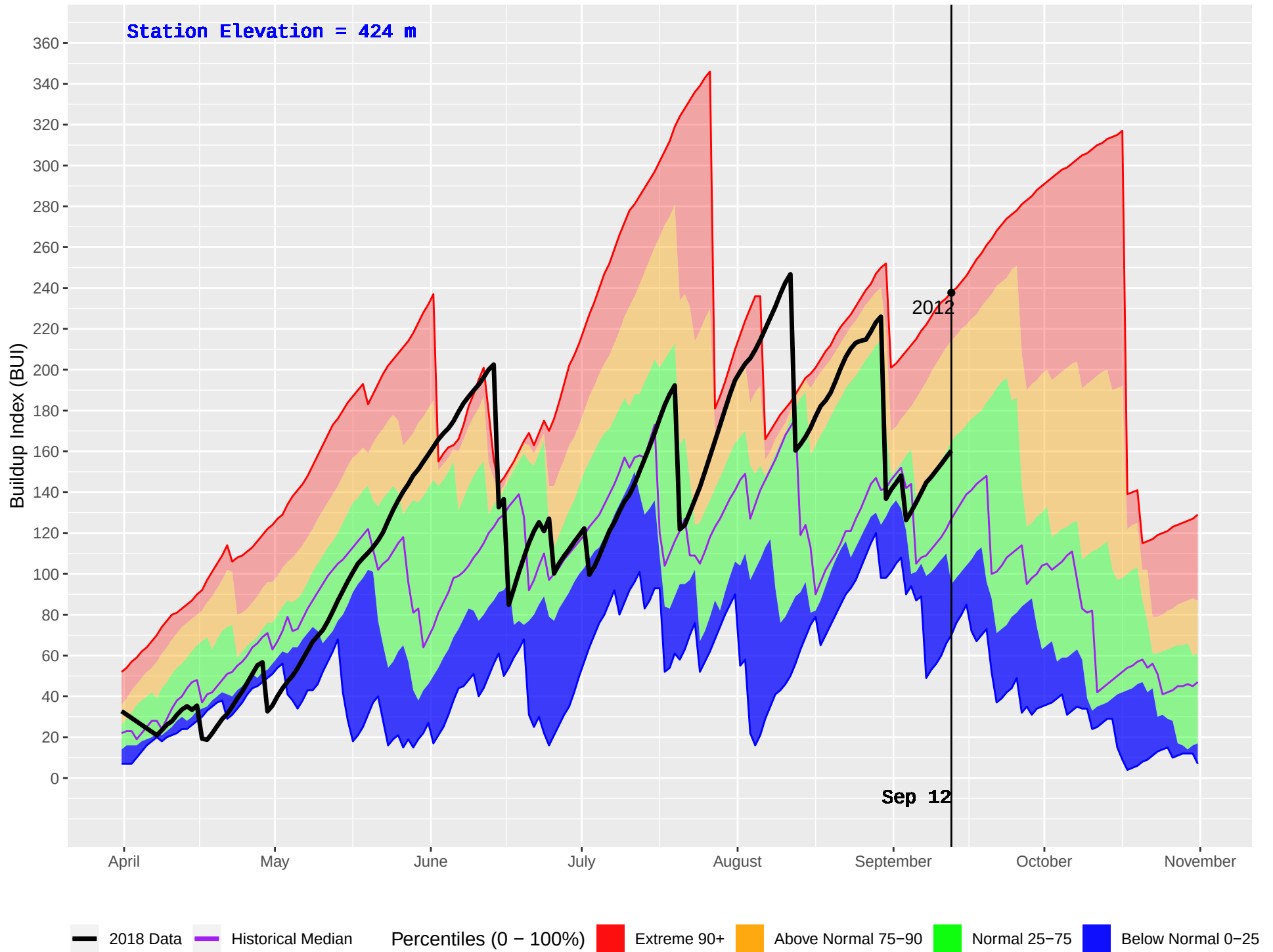
SPLINTLUM (1055) : Historical (2009–2016) and Current (2018) Daily Buildup Index (BUI)
